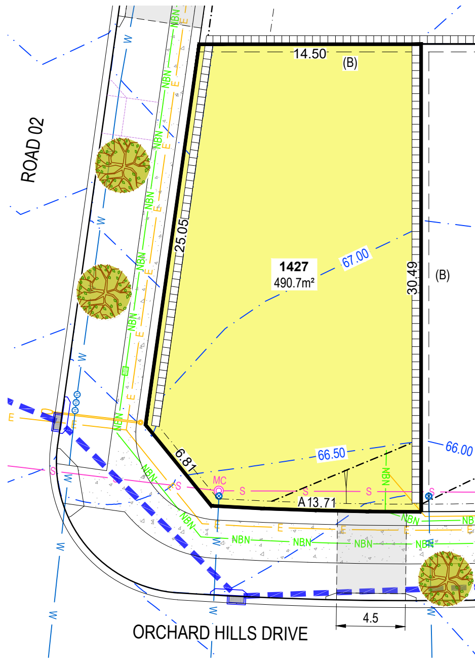
(B) PROPOSED EASEMENT FOR RETAINING WALL SUPPORT 0.5m WIDE
